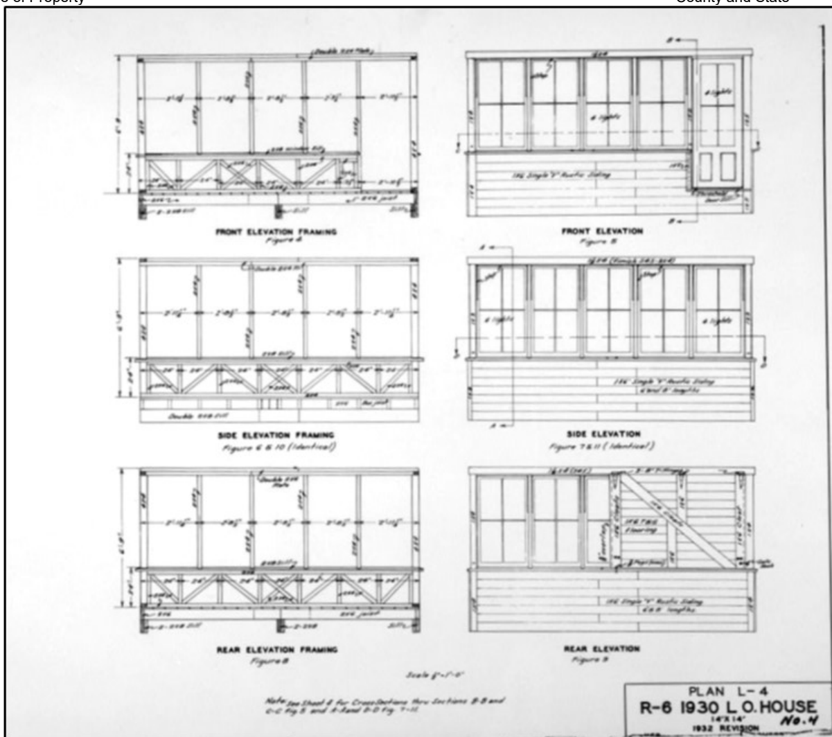
MT_RosebudCounty_PokerJimButteLookout_0015. Lookout House Plan L-4, Sheet 4 of 7, Site 24RB2233, Poker Jim Butte Fire Lookout L-4 Construction Plan, 1932 revision
